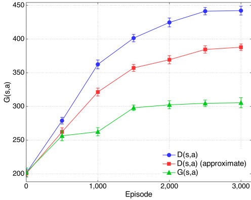
Figure 1: Rover domain results (10 agents). Approximating D_i(s, a) results in 88% of the performance attained when analytically computing D_i(s, a) . Approximating the difference evaluation function results in significant performance gains when compared to using the system evaluation function G(s, a) .
