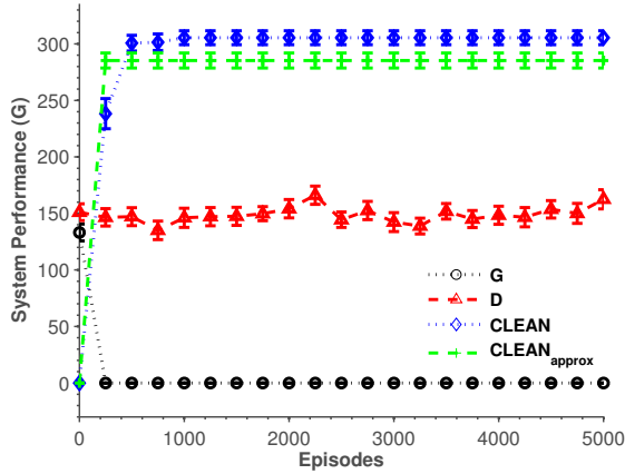
Figure 5: GSD results with 1000 agents, where agents can select from 15 available actions, the standard deviation of the objective function \sigma is 400, the mean of the objective function \mu is 200, the learning rate \alpha_1 is 0.1, the update rate for agents' function approximators is 0.1, and the exploration rate \epsilon is 0.1. Approximate CLEAN rewards significantly outperform both global and difference rewards, and provide 94% of the performance of directly computed CLEAN rewards.
