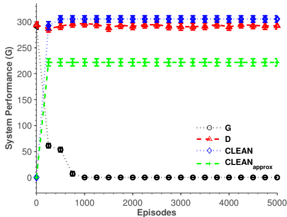
Figure 6: GSD results with 1000 agents, where agents can select from 10 available actions, the standard deviation of the objective function \sigma is 400, the mean of the objective function \mu is 200, the learning rate \alpha_1 is 0.1, the update rate for agents' function approximators is 0.1, and the exploration rate \epsilon is 0.1. Approximate CLEAN rewards significantly outperform global rewards, but only achieve 75% of the performance of directly computed CLEAN rewards, and 78% of the performance of difference rewards.
