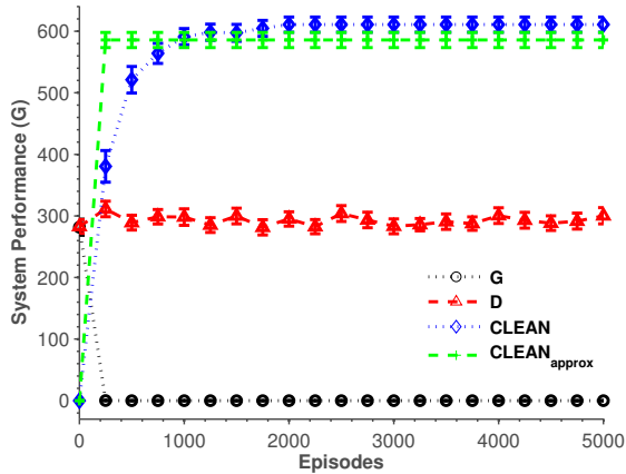
Figure 8: GSD results with 2000 agents, where agents can select from 15 available actions, the standard deviation of the objective function \sigma is 400, the mean of the objective function \mu is 200, the learning rate \alpha_1 is 0.1, the update rate for agents’ function approximators is 0.1, and the exploration rate \epsilon is 0.1. Approximate CLEAN rewards significantly outperform both global and difference rewards, and provide 96% of the performance of directly computed CLEAN rewards.
