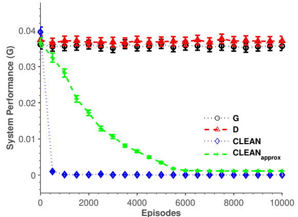
Figure 2: DCP results with 1000 agents, where \epsilon = 0.01 , \sigma = 1 , \alpha_1 = 0.005 , and \alpha_2 = 0.001 . Approximated CLEAN rewards outperform difference rewards and global rewards, and achieve 98% of the improvement over difference evaluations that the analytically computed CLEAN rewards attain.
