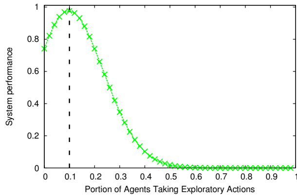
Figure 1: Demonstration of exploratory action noise: agents learned for 1000 episodes with \epsilon -greedy action selection where \epsilon = 0.1 . After learning, the policies are fixed, and we test performance of the learned policies under different amounts of exploration (some agents' policies are replaced with random exploratory policies). Agents perform better in the presence of exploration than they do with no exploration. The highest system performance is when the exploration rate is near \epsilon , because agents have learned policies which are biased to include this level of random exploration by other agents in the system.
