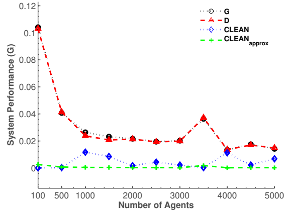
Figure 4: DCP results: Scaling. Regardless of system size, approximate CLEAN rewards outperform global and difference rewards, and outperform directly computed CLEAN rewards in some cases.
