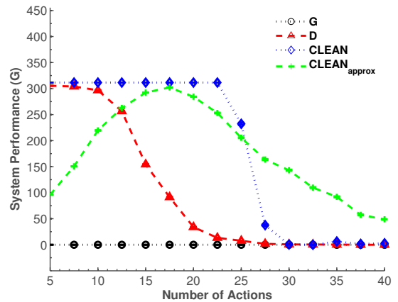
Figure 7: GSD results: scaling the number of actions.
