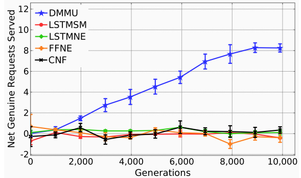
Figure 2: Comparative performance in the cybersecurity task. The server fleet consists of 10 proxy servers handling a request volume of 100 from 20 distinct devices. A random number of devices between {7,13} out of 20 are nefarious while the rest are genuine. Asynchronous memory access by agents with the busy period following each action set randomly set between {0,2} timesteps.
