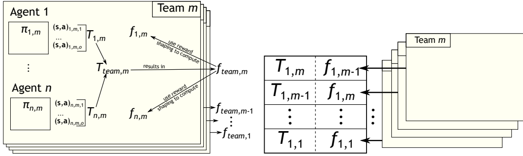
(a) A team m of n agents executes their policies (\pi_{1,m}, \dots, \pi_{n,m}) . The team's joint-trajectory T_{team,m} receives a score of f_{team,m} . Reward shaping can be applied to f_{team,m} to generate shaped feedback values (f_{1,m}, \dots, f_{n,m}) . This process is repeated for all the m episodes in each evolutionary algorithm (EA) generation.
