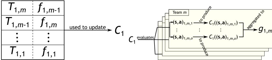
(c) Once per generation, our method uses the mapping between the trajectories and shaped feedback to update Agent 1's intermediate critic ( C_1 ), which is a functional model. Our method repeats this process for all other agents.
