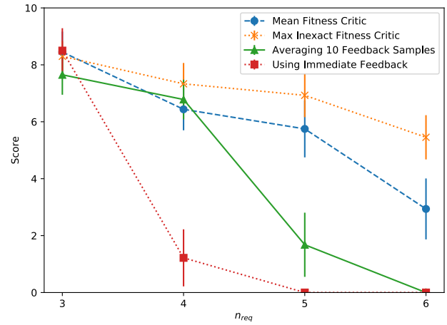
Figure 7: Mean performance scores for teams of agents trained with and without fitness critics. Agents are trained with CCEA on the tightly-coupled multi-rover domain with 15 rovers, 4 points of interests (POIs), and various degrees of coupling ( n_{req} ). Error bars denote 95% confidence interval.
