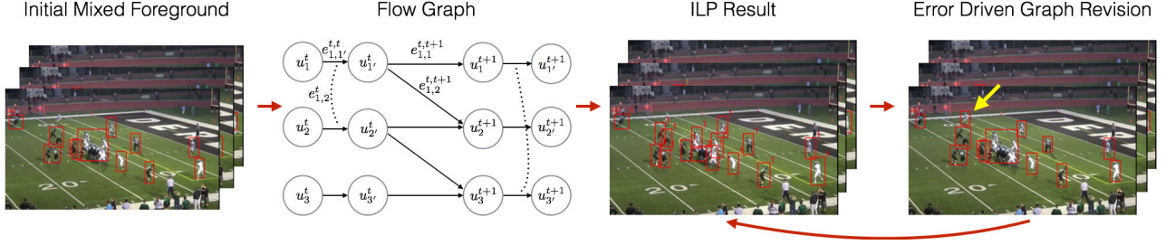
Figure 2: System Overview. First extract noisy foreground by running an object detector and foreground segmentation. A flow graph is then built and transformed into an integer program. In the following iterations, the approach detects places where integrity/domain constraints are violated by the current solution and applies one or more graph-revision operators to obtain a new graph and updated solution.
