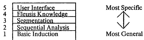
Figure 4. Layered Structure of Eleusis Program.
