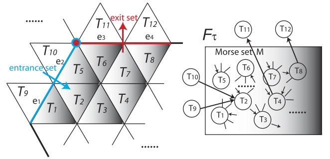
Fig. 9. This illustrates the classification of boundary edges. The image to the left provides a portion of the mesh with a Morse set M inside the shadow region. The image to the right provides the configuration of a discrete map (i.e., a flow combinatorialization) \mathcal{F}_\tau . Note that we ignore the inner configuration of the graph inside the Morse set M because it does not affect the classification.
