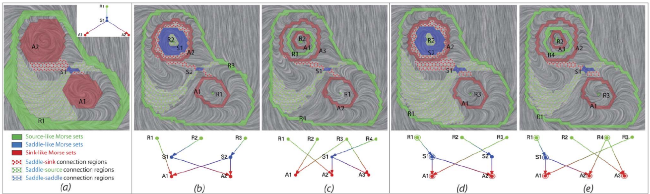
Fig. 1. The MCGs of an analytic vector field using the geometry-based method (a), the global computation ((b): \tau = 0.1 and (c) \tau = 0.2 ), and our hierarchical refinement framework ((d): \tau_{max} = 0.1 and (e) \tau_{max} = 0.2 ). Our refinement method takes 10.11 seconds for \tau_{max} = 0.2 , while the global method uses 22.88 seconds with the same \tau value. Note that our refinement method obtains comparable results to the global method but with a more coherent representation of the topology. This is because the global method relabels all the Morse sets after each computation, while our hierarchical refinement modifies only one Morse set (one node of the graph) after each iteration starting from the MCG shown in (a). In particular, in (d) R3 is obtained from the refinement of A1 in (a), S2 and R2 are from A2 in (a). In (e), R4 and A3 are the results of refining S2 in (d). In addition, we point out that the MCG in the left visualization (a-c) lacks the ability to distinguish between a source-like Morse set and a periodic orbit-like source Morse set (e.g., R1 and R4 ). The new Morse set classification and visualization based on the Conley index provides such information.
