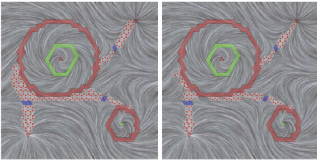
Fig. 8. This figure shows the connection regions before (left) and after refinement (right).
