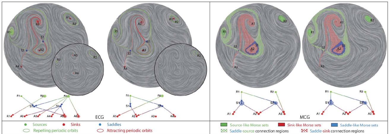
Fig. 3. This figure provides the ECGs [1] (left) and MCGs [2] (right) of a cross section of a diesel engine simulation. This cross section is cut at the 25 percent of the length of the cylinder from the top where the intake ports meet the chamber. The images to the left show two ECGs computed using the Runge-Kutta integration scheme [24] of the second order (RK2) and of the fourth order (RK4), respectively. The two inlets show the detected periodic orbits under different integration schemes. As can be observed, ECGs are numerically unstable and can provide misleading information. As a comparison, the MCGs of the same field are computed using RK2 (middle-right) and RK4 (right-most), respectively. Despite the different sizes of the Morse sets in the two MCGs, their topological graphs are identical, indicating the stable extraction of these features. We refer the readers to [2] for a more detailed discussion.
