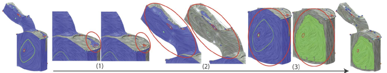
Fig. 12. This figure illustrates the refinement process of the MCG from a gas engine simulation. Left-most shows the MCG of a geometry-based approach. From (1-3), we refine the circled Morse set with \tau = 0.2, 0.4 , and 0.4 , respectively. The MCG obtained using a global \tau = 0.4 shows the similar result (right-most). The color coding is provided in Fig. 1.
