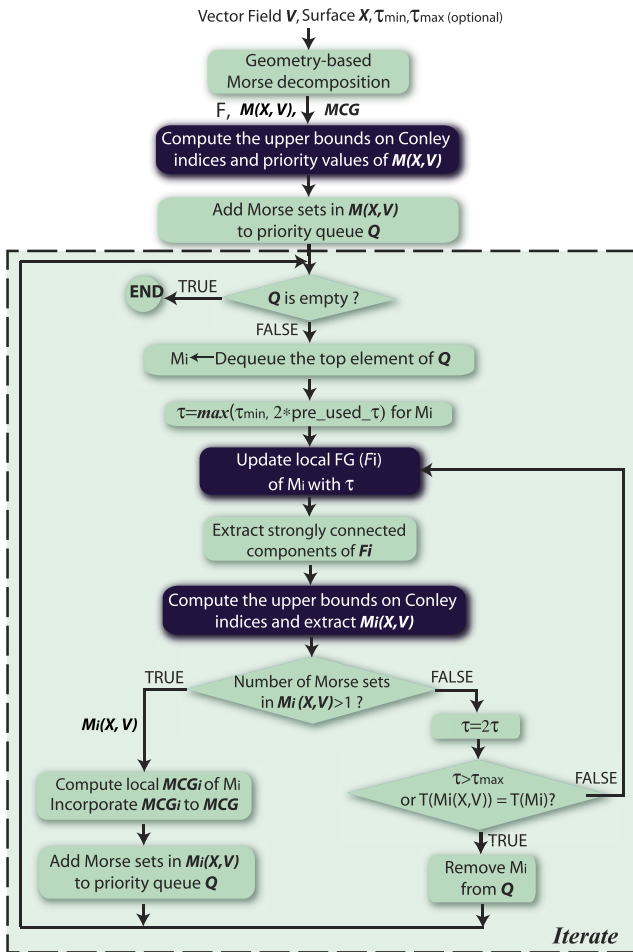
Fig. 7. The pipeline of the proposed locally hierarchical refinement of Morse decompositions of vector fields. Note that the highlighted modules are the focus of this paper (Section 5 for local refinement, Section 6 for Conley index computation, and Section 7 for the computation of the priority values).
