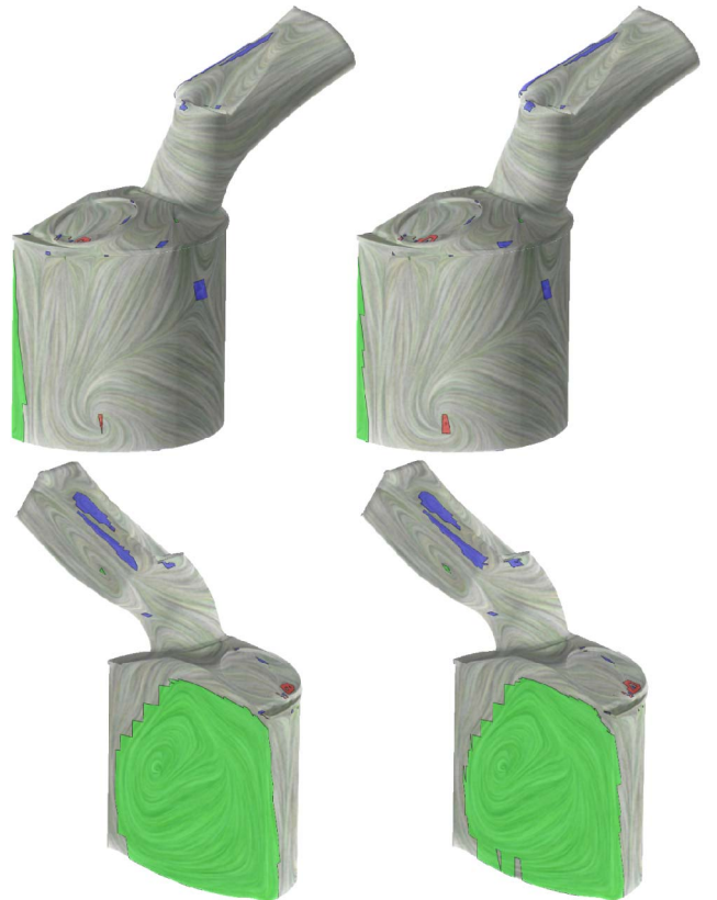
Fig. 13. This figure shows the results of the Morse decompositions of a gas engine simulation data set using a global method (left column), and the present automatic refinement (right column). Both methods employ \tau_{max} = 0.4 . Note that both methods produce comparable decomposition with a slight difference of the shapes and sizes of the obtained Morse sets. The color coding is provided in Fig. 1.
