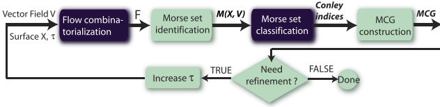
Fig. 4. The MCG computation pipeline using Morse decomposition. Note that the modules colored in black are the focus in this paper. More specifically, we introduce the idea of local flow combinatorialization and provide an efficient algorithm for the computation of an upper bound of the Conley index.
