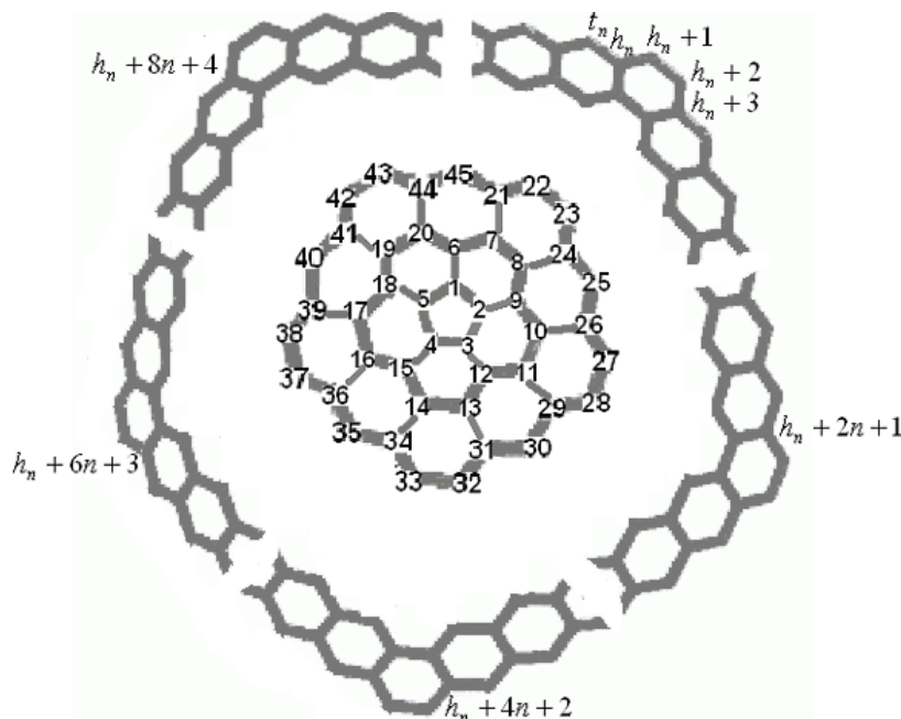
Fig. 1. The One-Pentagonal Carbon Nanocone CNC_5[4] .
