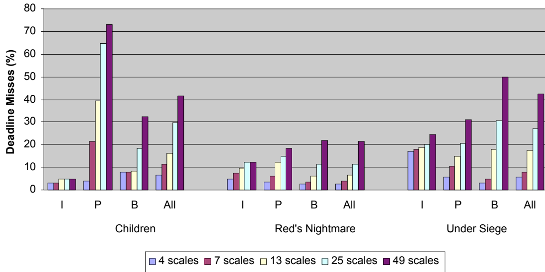
Figure 17: Percentage of the deadlines misses for different processor settings for FDCA.
