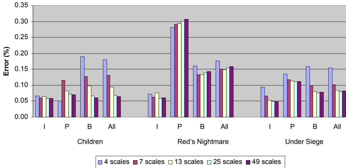
Figure 12: Errors for various processor settings for Dynamic method.
