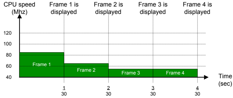
(a) With DVS (Ideal)
