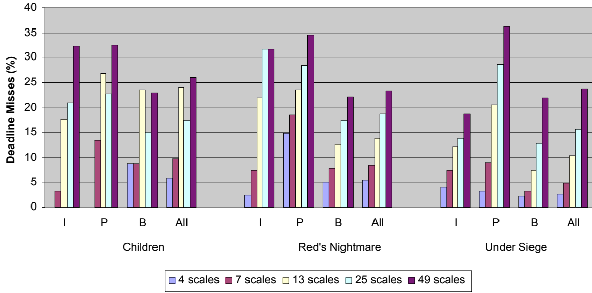
Figure 16: Percentage of the deadlines misses for different processor settings for Dynamic.
