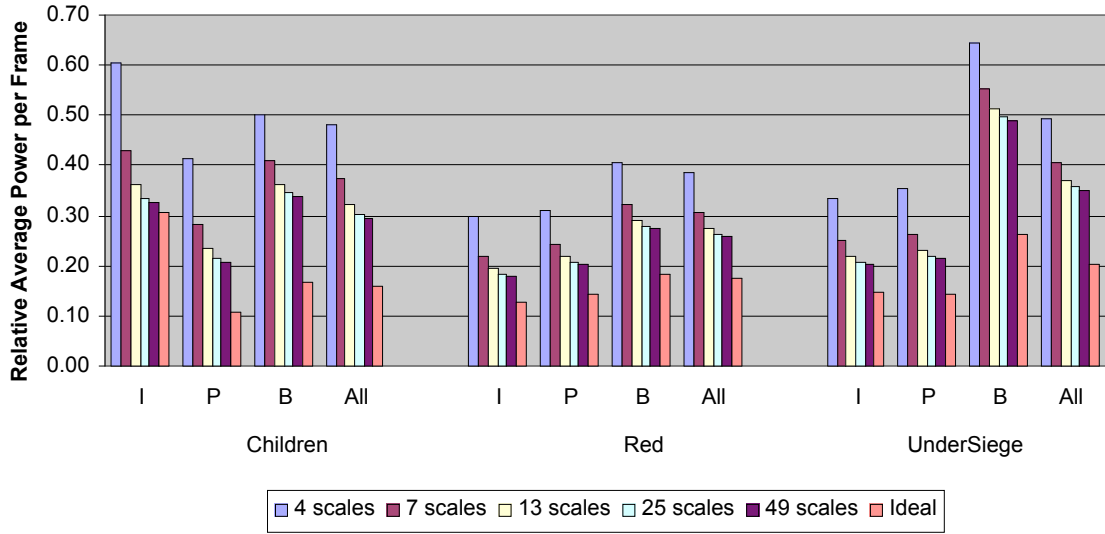
Figure 13: Relative average power per frame for various processor settings for FDCA method.
