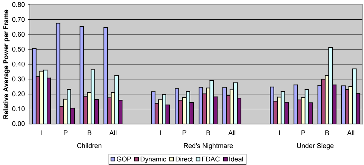
Figure 9: Relative average power consumption per frame for various DVS approaches.
