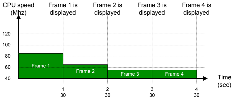
(b) With DVS (Ideal)
