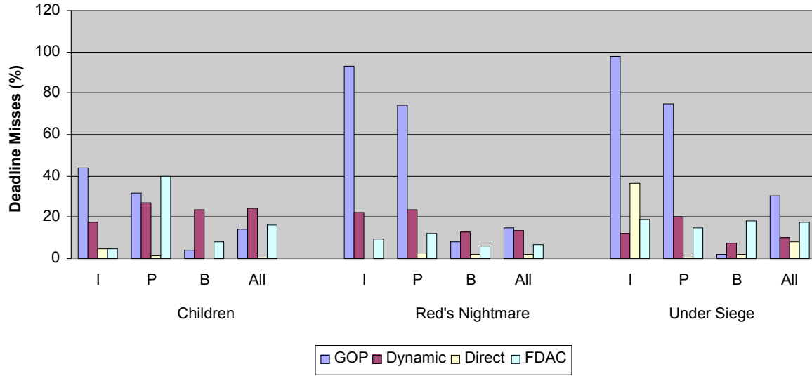
Figure 15: Percentage of deadline misses for various DVS approaches.
