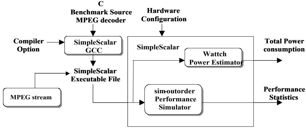
Figure 7: Simulation environment.
