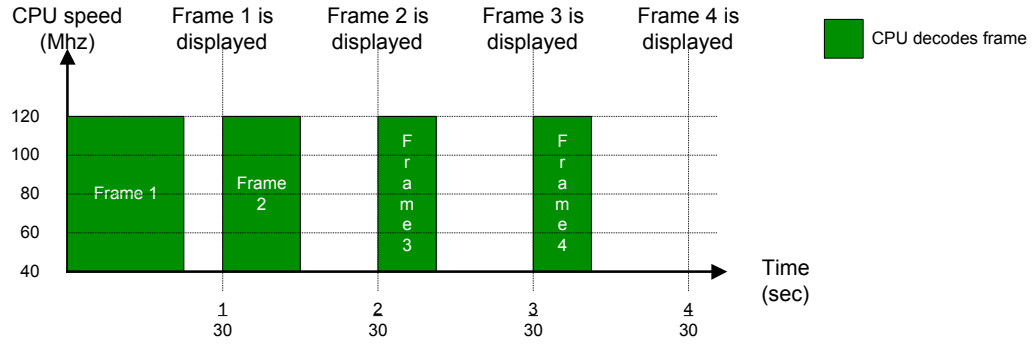
(a) Without DVS.
