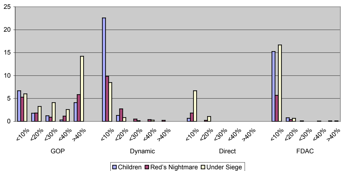
Figure 18: The degree of deadline misses for various DVS approaches.
