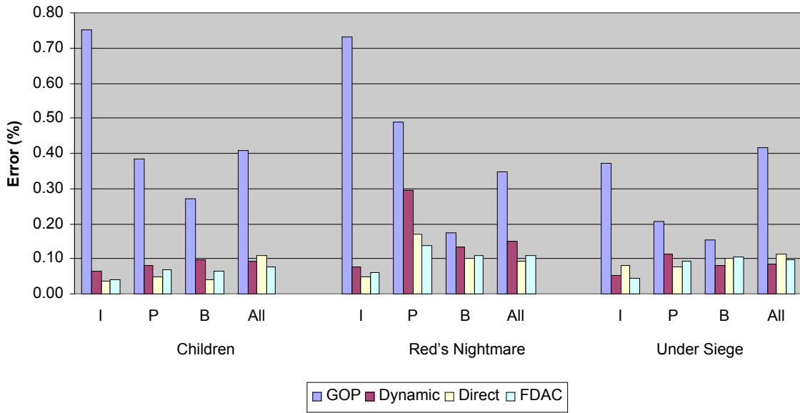
Figure 10: Errors for various DVS approaches.
