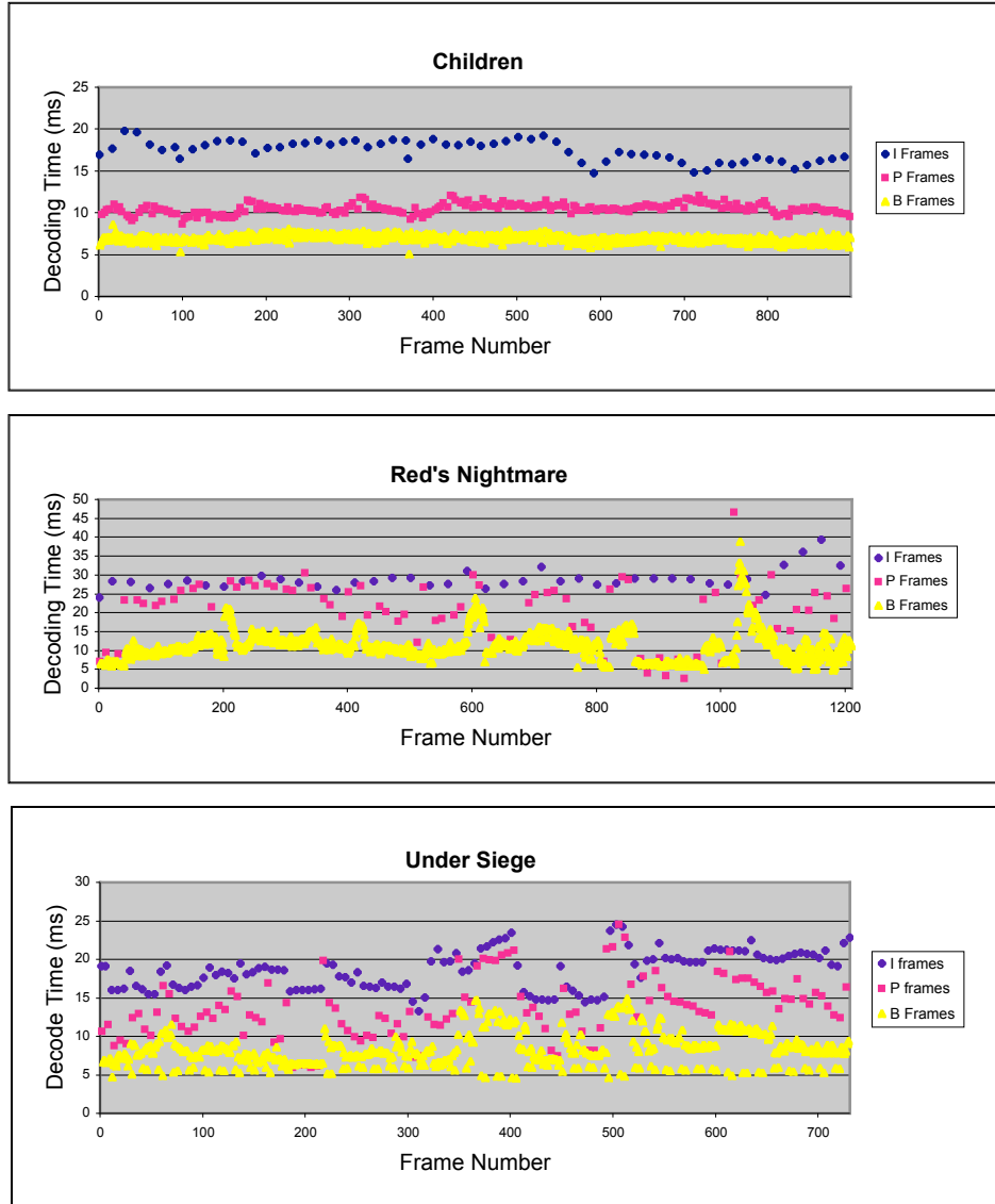
Figure 8: Frame decoding times for each clip.
