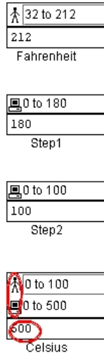
Figure 5. An assertion conflict in Forms/3. The user wrote the assertion on the Celsius cell (0 to 100), which conflicts with the computer generated assertion (0 to 500). This prompts the user to check for errors in the cells' formulas [Burnett et al. 2003]. Original figure obtained from authors.
