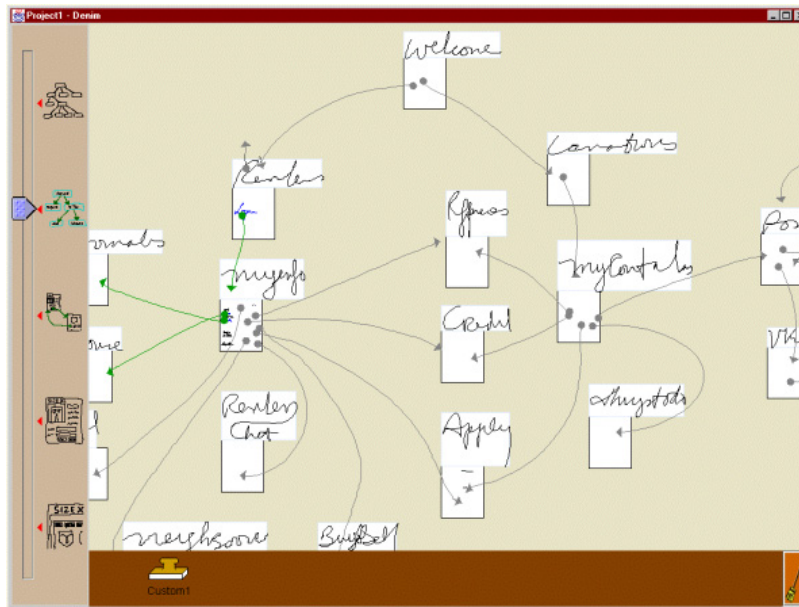
Figure 2. Links between web site content, sketched in DENIM, an informal web site sketching tool. Reprinted from [Newman et al. 2003] with permission from authors.
