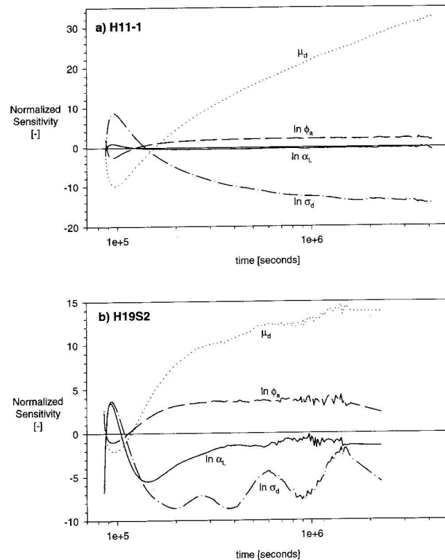
Figure 5. Normalized sensitivity for estimated parameters of multirate diffusion model at (a) H11-1 and (b) H19S2.
