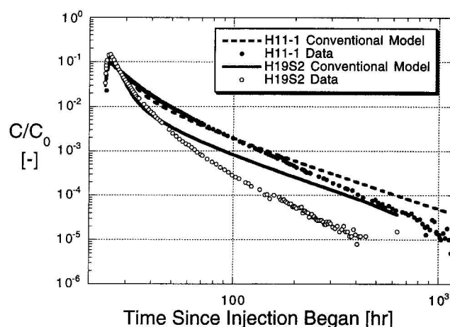
Figure 2. Best fits of conventional double-porosity models to the H11-1 and H19S2 data. Parameters are given in Table 2.
