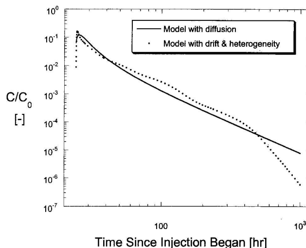
Figure 6. Best fit of multirate diffusion model to SWIW model incorporating both heterogeneity and drift.
