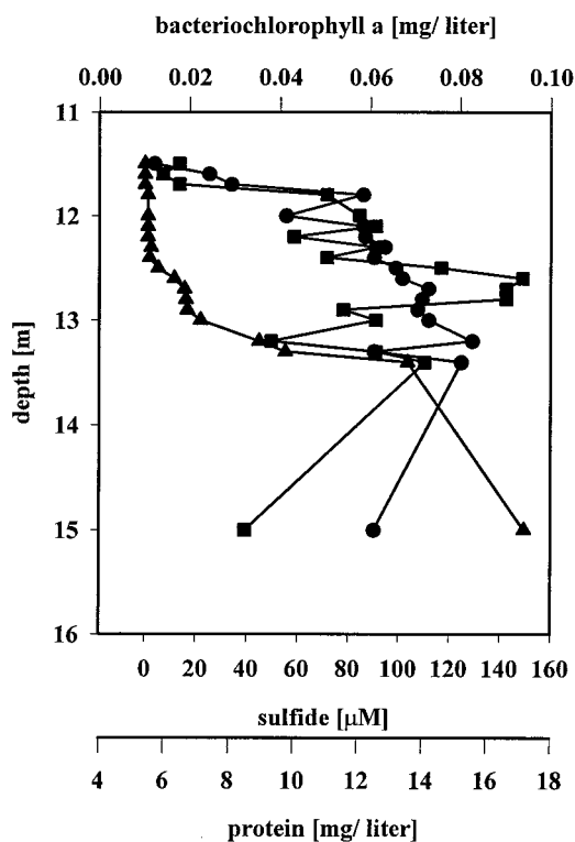
FIG. 3. High-resolution profiles (22 July 1998, afternoon) of bacteriochlorophyll a (●), protein (■), and sulfide (▲) in the redoxcline.
