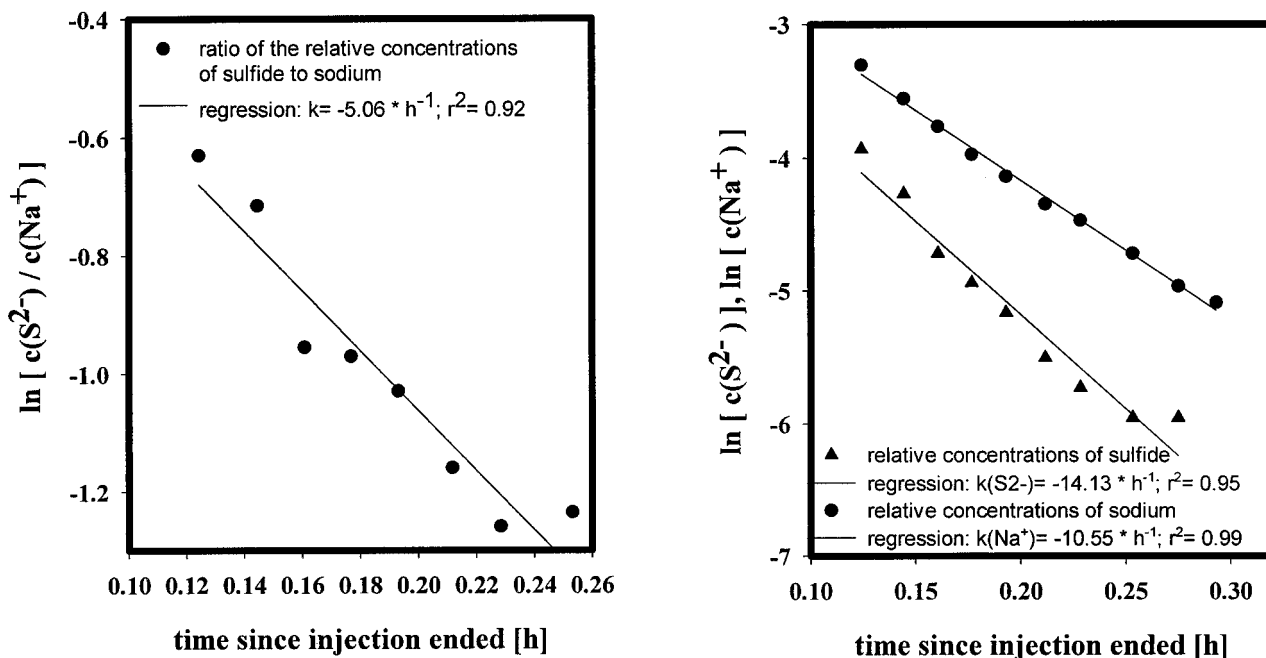
FIG. 4. (Left) Breakthrough curve during the extraction (19 September 1997). Conditions: 600-ml test solution; pump rate during retrieval, 40 ml · min -1 . (Right) Tracer (Na + ) and reactant (S 2- ) breakthrough curves during the extraction phase (19 September 1997). Conditions: 600-ml test solution; pump rate during retrieval, 40 ml · min -1 .
