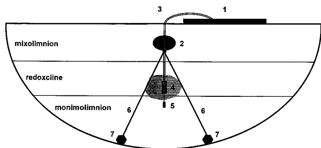
FIG. 1. Installation for push-pull test experiments in Lake Cadagno. 1, working platform; 2, underwater buoy; 3, tube; 4, distributor; 5, weight; 6, cable; 7, buoy stones.
