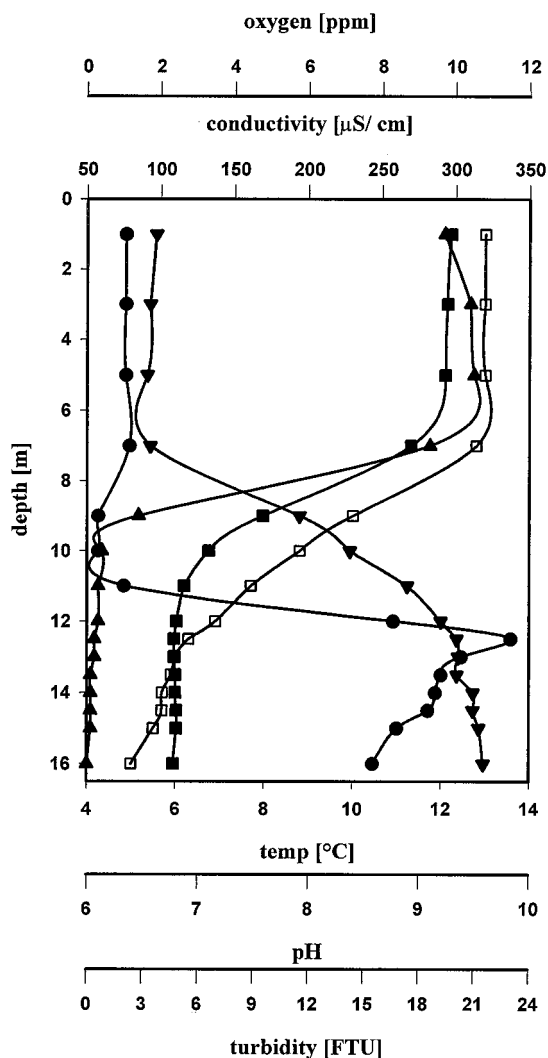
FIG. 2. Different profiles of Lake Cadagno (17 September 1997, morning). Profiles for conductivity (▼), oxygen (▲), temperature (□), turbidity (●), and pH (■) are shown.
