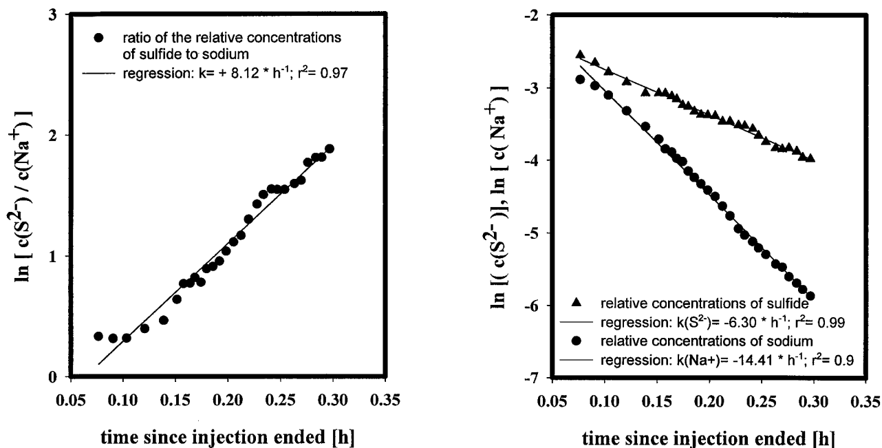
FIG. 5. (Left) Breakthrough curve during the extraction phase (6 October 1997). Conditions: 600-ml test solution; pump rate during retrieval, 40 ml · min -1 . (Right) Tracer (Na + ) and reactant (S 2- ) breakthrough curves during the extraction phase (6 October 1997). Conditions: 600-ml test solution; pump rate during retrieval, 40 ml · min -1 .
