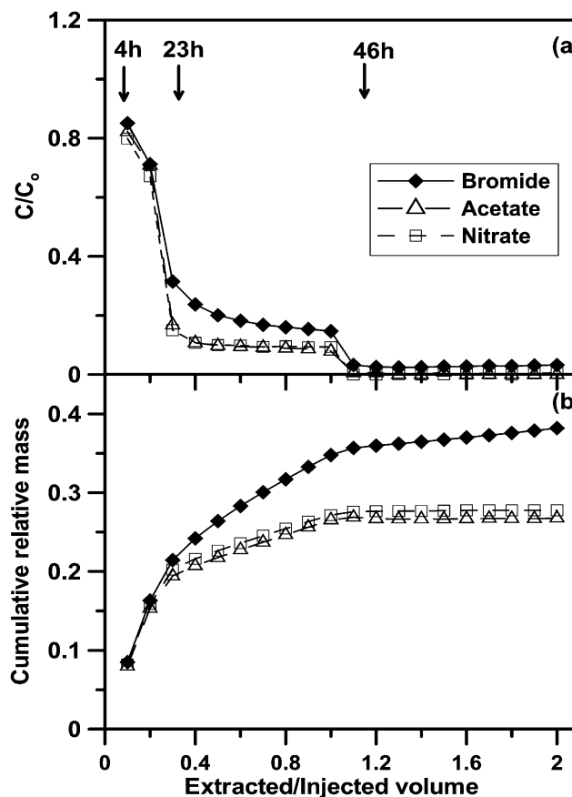
Fig. 1. Breakthrough curves showing (a) relative concentrations and (b) cumulative relative mass (i.e. cumulative mass extracted/total mass injected) recovered for \text{Br}^- , \text{NO}_3^- and acetate during the PPT vs. the relative cumulative extracted volume (cumulative volume extracted divided by the total injected volume of test solution). Arrows indicate the starting time of the three extractions.
