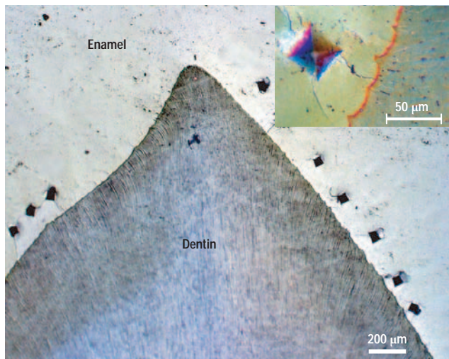
Figure 2 Optical micrograph of the placement of Vickers indents in the enamel. The indents were within ~20–50 μm from the optical DEJ in a human molar, which were used to create cracks that impact upon the DEJ. Inset shows optical micrograph with Nomaski interference contrast of one such indentation with cracks, which emanate from the indent corners, propagating into the scalloped interface.
