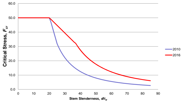
Stem Local Buckling of Tees
