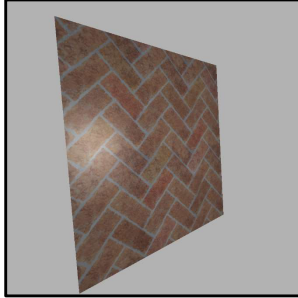
Ordinary Texture
