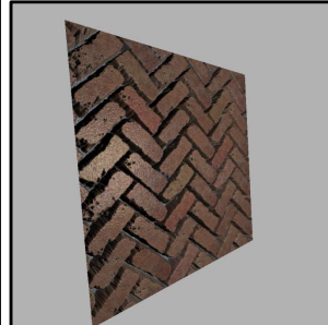
Parallax Mapping
