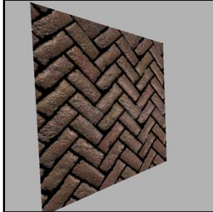
Normal-Mapping
