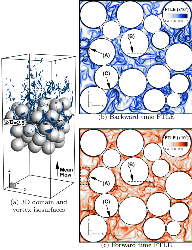
FIG. 10. Flow through the random sphere pack. (a) Shows the simulation domain and instantaneous isosurfaces of \lambda_{ci}/\lambda_{ci}^{max} = 0.25 , and the z/D = 2.5 plane used for visualization of the FTLE fields. (b) and (c) show a snapshot of the FTLE fields for at the z/D = 2.5 cross stream slice. The LCS candidates in pores A, B, and C demonstrate distinct, time dependent behavior.
