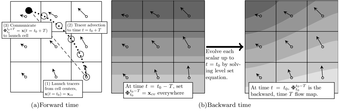
FIG. 1. Lagrangian and Eulerian computations of the flow maps for time t = t_0 . (a) The Lagrangian computation of the forward time flow map, \Phi_{t_0}^{t_0+T} . (b) The Eulerian computation of the backward time flow map, \Phi_{t_0}^{t_0-T} . The scalar field shows the evolution of the y component of the backward time flow map in a simple velocity field.
