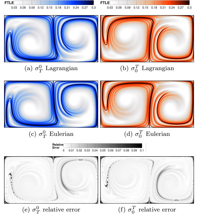
FIG. 5. Comparison of the Lagrangian and Eulerian approaches to calculating the FTLE field. (a) through (d) show the FTLE fields computed in (a) backward time with the Lagrangian approach, (b) forward time with the Lagrangian approach, (c) backward time with the Eulerian approach (d) forward time with the Eulerian approach. (e) and (f) show the relative error between the Lagrangian and Eulerian approaches for backward and forward time respectively.
