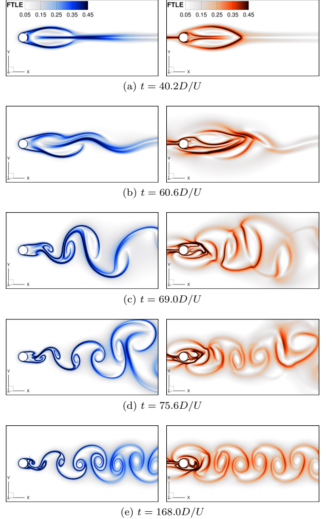
FIG. 7. Snapshot of FTLE fields for flow over a cylinder at Re = 300 for T = 7.8D/U . Left column shows backward time FTLE, right column shows forward time FTLE.
