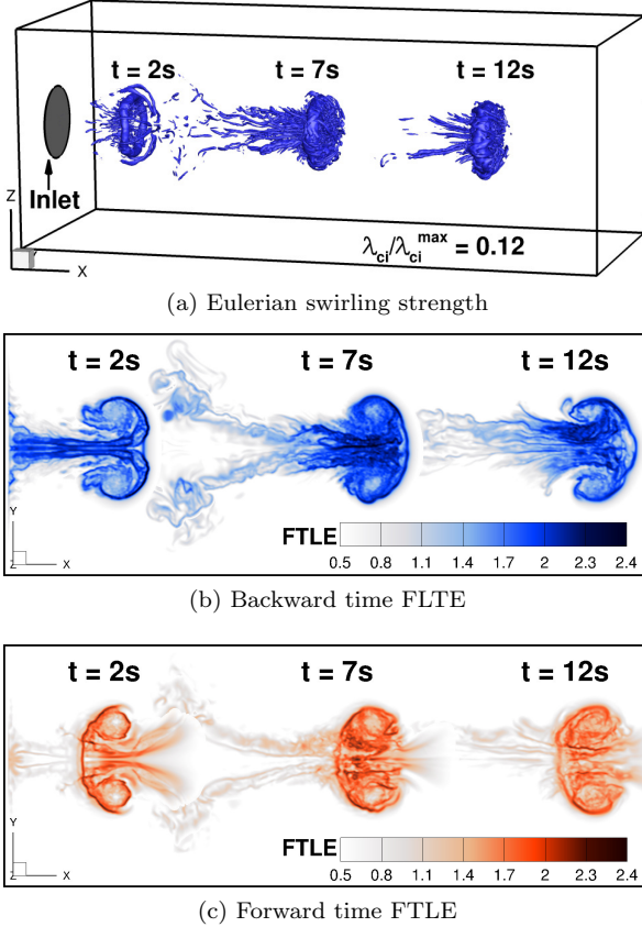
FIG. 9. Snapshots of the three dimensional vortex ring at t = 2s, 7s, 12s . (a) Isosurface of swirling strength, \lambda_{ci}/\lambda_{ci}^{max} = 0.12 . (b-c) FTLE fields for the z = 0 cross sectional slice through the center of the 3D vortex ring
