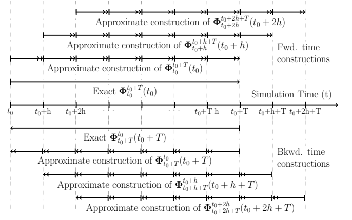
FIG. 2. Integration of the flow map composition scheme with the flow solver forward time advancement. At any simulation time t which is a multiple of h , the forward time flow map, \Phi_{t-T}^t(t-T) , and the backward time flow map, \Phi_t^{t-T}(t) , are constructed from the N time h sub-steps.
