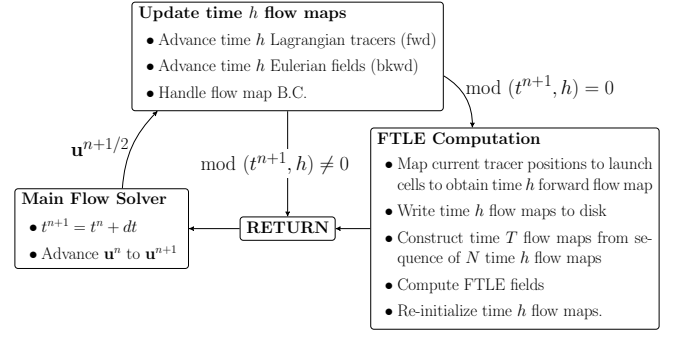
FIG. 3. Block diagram showing the flow of the CFD simulation with integrated FTLE computations.
