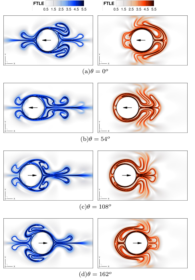
FIG. 8. FTLE fields for selected phase angles in one half cycle of the oscillating cylinder flow. The arrow denotes the direction of cylinder motion. Left column shows backward time FTLE, right column shows forward time FTLE.
