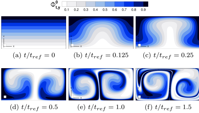
FIG. 4. Evolution of the Eulerian representation of the backward time flow map on the fixed grid during simulation of the double gyre flow. The scalar field, \Phi_{t,y}^0 , represents the y coordinate of the Lagrangian particle at time, t = 0 , which arrives at the fixed grid points at each later time.
