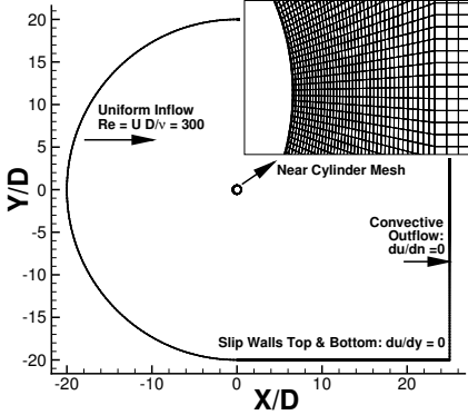
FIG. 6. Domain and mesh used for simulating flow over a fixed cylinder.
