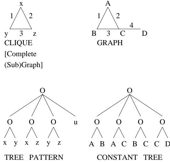
Figure 15. CLIQUE as Unordered Tree
