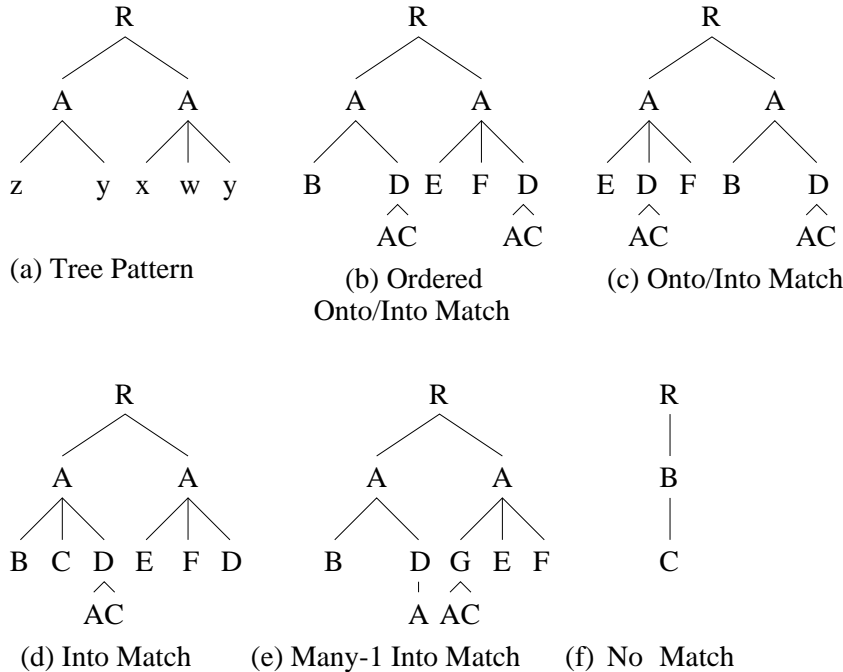
Figure 1. Match Semantics Example
