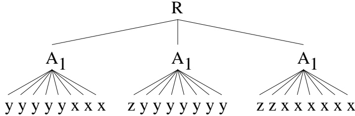
Figure 3. Sample UT target with n = 3 subtrees.
