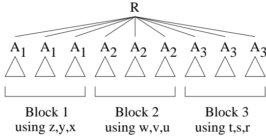
Figure 4. Sample UF Target for n = 3
