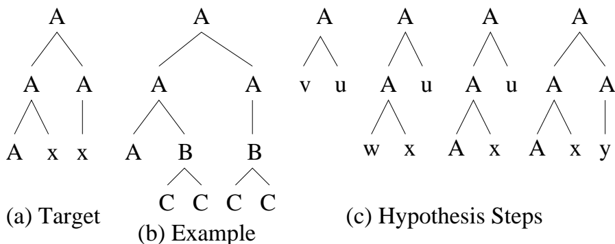
Figure 6. UT Learning Example
