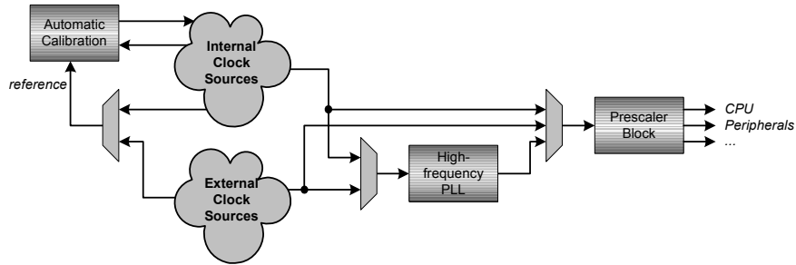
Figure 1-1. XMEGA Clock System Overview
