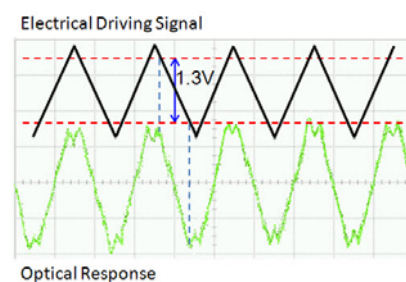
Figure.2 Low frequency modulation measurements showing a low V_{\pi} of 1.3V for the E-O polymer nano-photonic modulator with 340μm modulation arm
