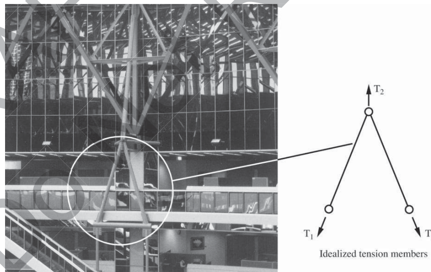
Figure 1.2 Use of Tension Members as Hangers
