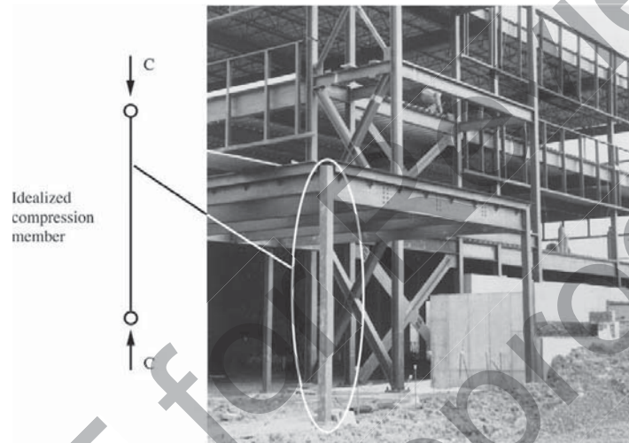
Figure 1.3 Use of Columns in a Building Frame
