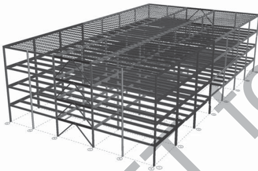
Figure 1.23 Three-Dimensional Computer Model of Complete Structure from RAM Structural System
