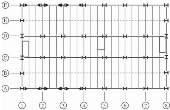
Figure 1.21 Representative First-, Third-, and Fourth-Floor Framing Plan
