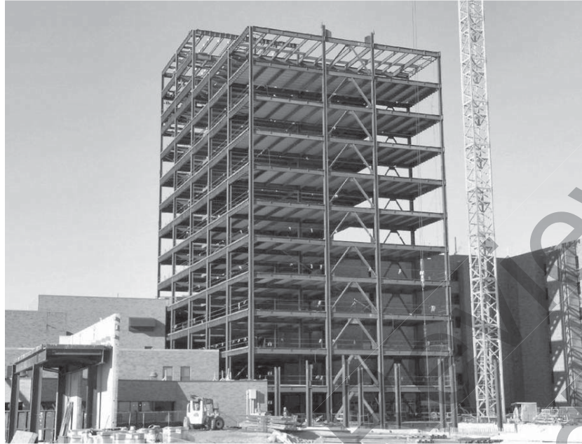
Figure 1.9 Braced Beam-and-Column Building Photo courtesy Douglas Steel Fabricating Corporation
