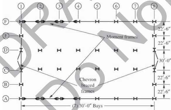
Figure 1.19 Schematic Plan for Integrated Design Problem
