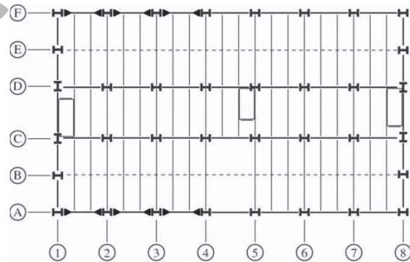
Figure 1.20 Representative Second-Floor Framing Plan
