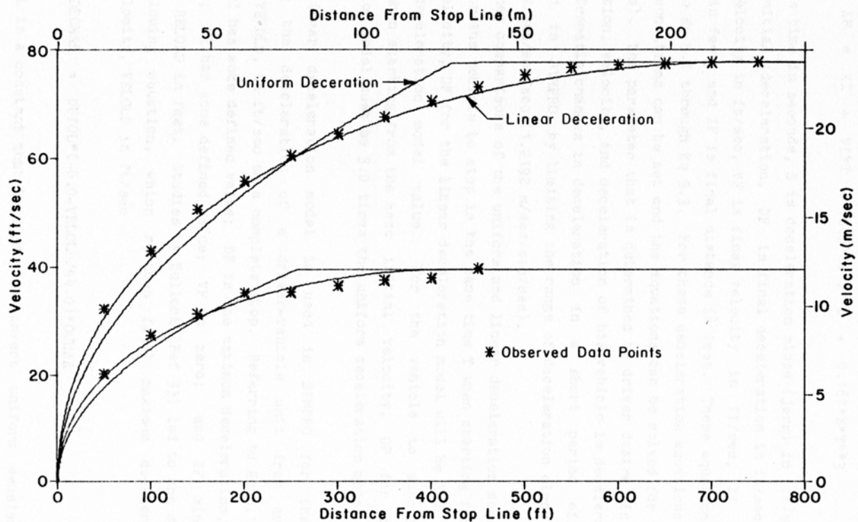
Figure 3 – Uniform versus Linear Deceleration and Observed Data
