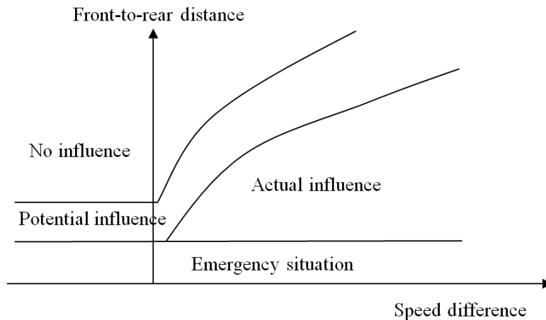
FIGURE 4 Thresholds and distances defining actual and potential influence areas in Willmann lane changing model (Source: Wiedmann and Reiter 1992).
