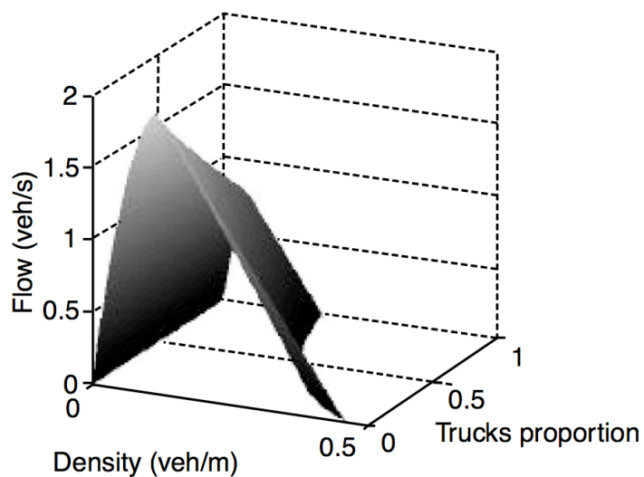
FIGURE 8 3 dimensional fundamental diagram where a high trucks proportion leads to lower speeds and flows. Picture from [13].
