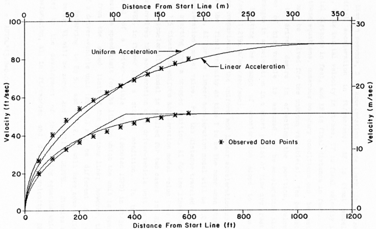
Figure 2 – Uniform versus Linear Acceleration and Observed Data
