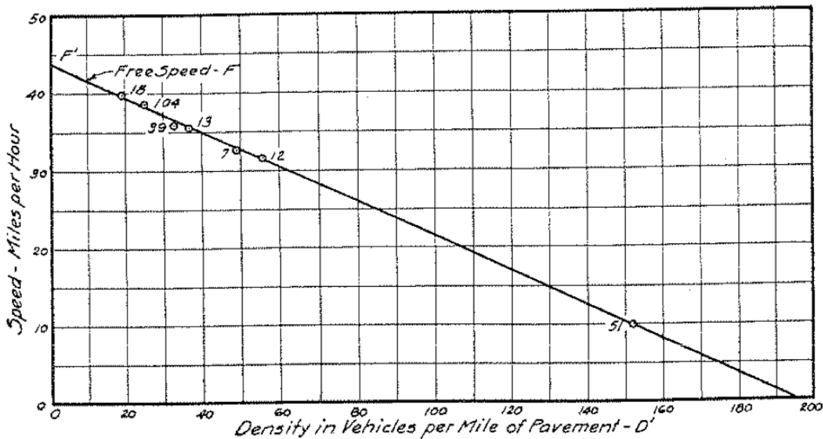
FIGURE 3 Greenshields' fundamental diagram (1935), showing a linear relation between density and speed. Picture from [4].
