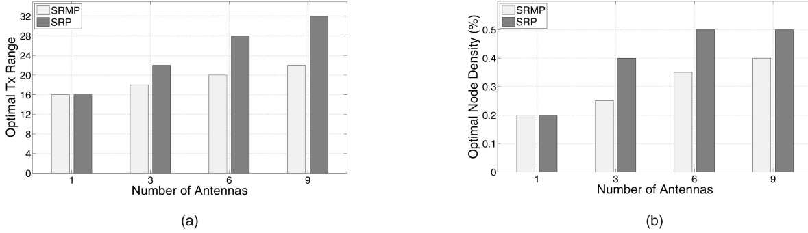
Fig. 7. Optimal design parameters under SRP and SRMP. (a) Optimal transmission range: nodeDensity = 0.5 percent. (b) Optimal node density: txRange = 30 m.
