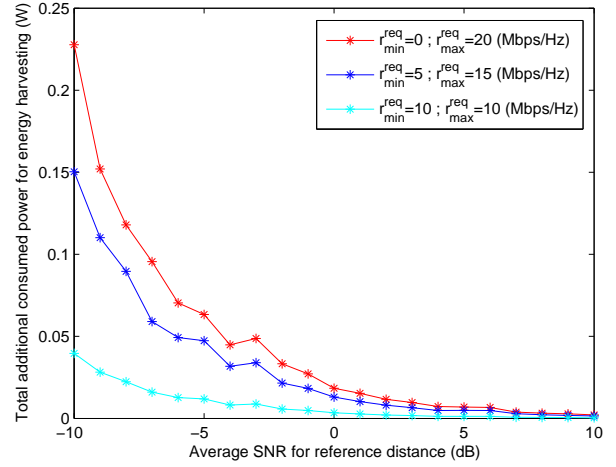
Fig. 4. Additional power cost with different data-rate requirements at the source nodes.
