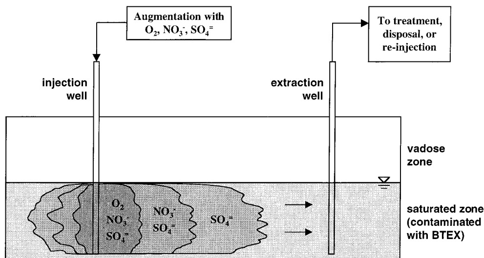
FIGURE 8. Representation of the geochemical zones that are expected to be established upon the combined injection of oxygen, nitrate, and sulfate.
