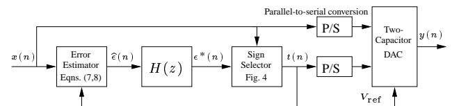
Figure 7: Mismatch-shaping two-capacitor DAC system.
