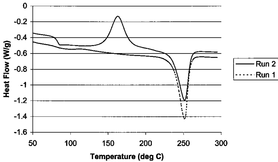
DSC Curve
