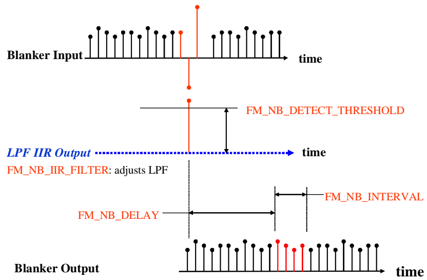
Figure 7. FM Noise Blanker
