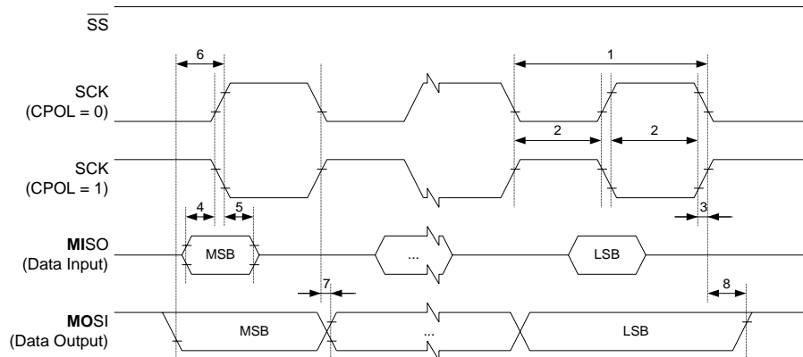
Figure 5. Timing Master Mode
