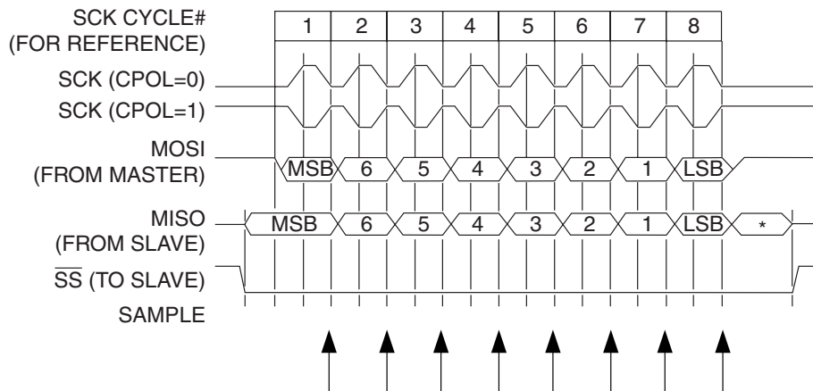
Figure 3. SPI Transfer Format with CPHA = 0
