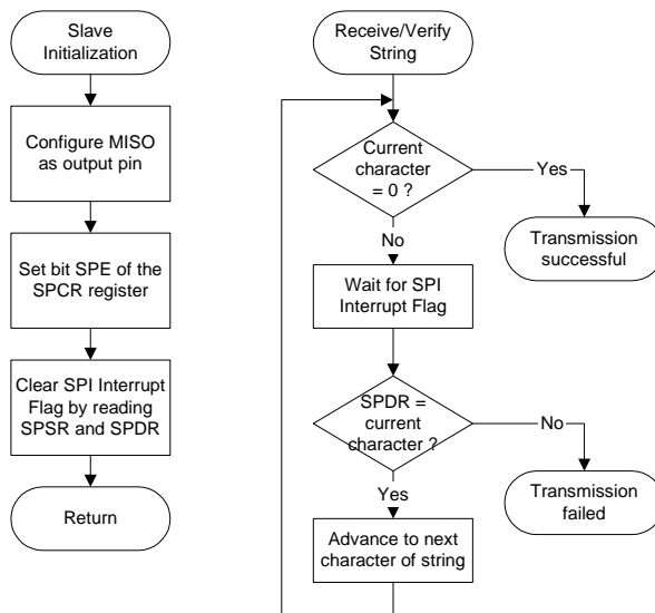
Figure 9. Polled slave - initialization and reception
