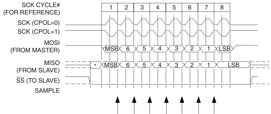
Figure 4. SPI Transfer Format with CPHA = 1
