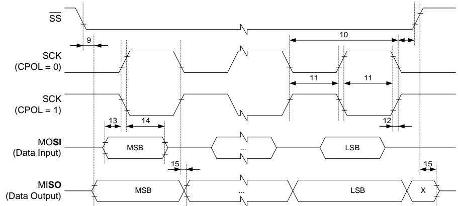
Figure 6. Timing Slave Mode
