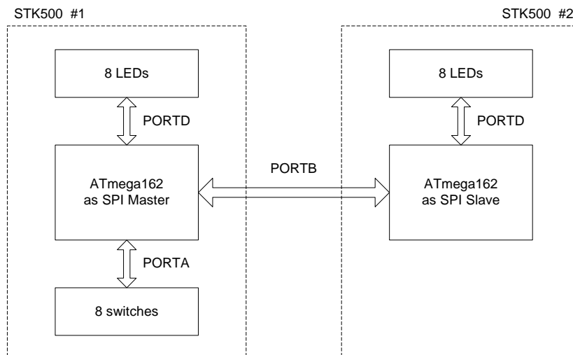
Figure 7. Hardware setup
