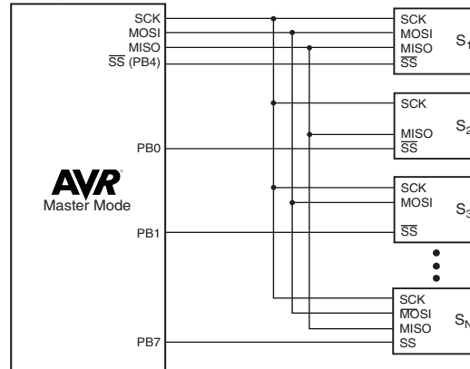
Figure 2. Multi Slave System
