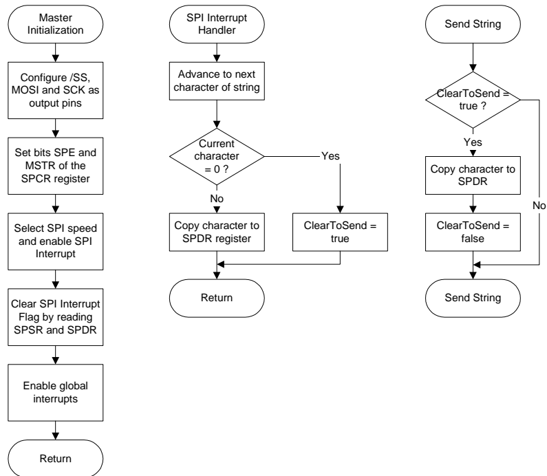
Figure 10. Interrupt controlled master - initialization and transmission
