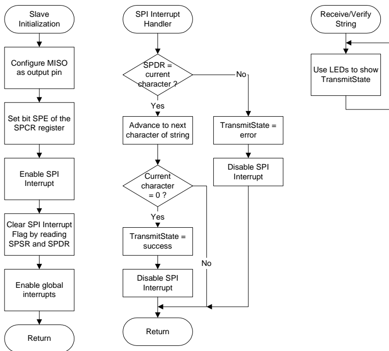
Figure 11. Interrupt controlled slave - initialization and transmission
