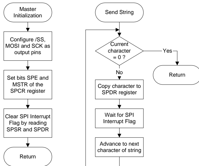
Figure 8. Polled master - initialization and transmission
