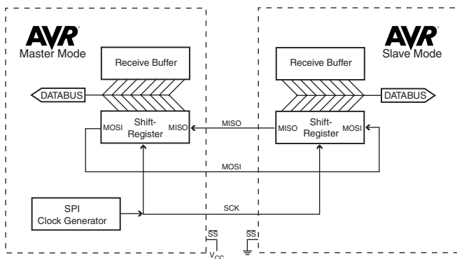
Figure 1. Master and Slave Interface.
